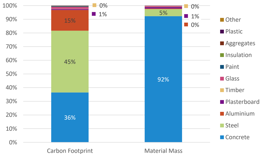
Figure 4-2: Carbon footprint and material mass breakdown for non-residential buildings over their full life (excl. biogenic CO 2 )
