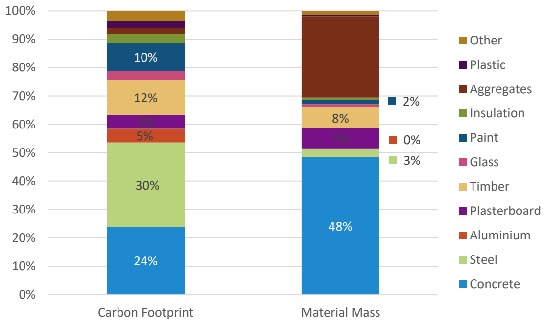
Figure 4-1: Carbon footprint and material mass breakdown for residential buildings over their full life (excl. biogenic CO 2 )
