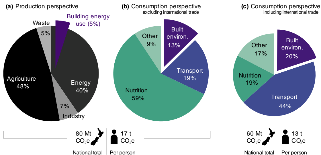
Figure 1-1: A breakdown of New Zealand’s carbon footprint in 2015 from: (a) a production perspective; (b) a life cycle consumption perspective excluding international trade; and (c) a life cycle consumption perspective including international trade (Vickers et al. 2018)
