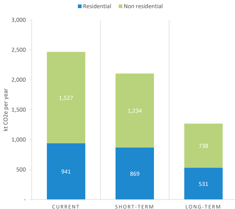
Figure 6-5: Carbon footprint comparison when short- and long-term improvements are applied (including biogenic carbon)
