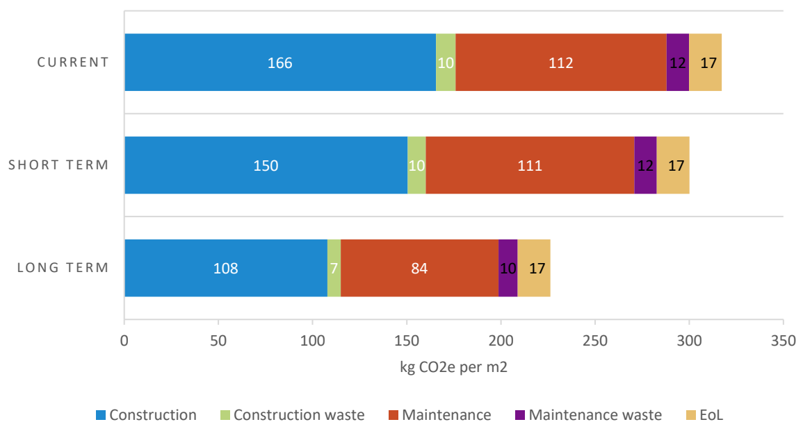
Figure 6-1: Breakdown of carbon footprint per 1 m 2 of gross floor area for residential builds, according to life cycle stage (excl. biogenic CO 2 )
