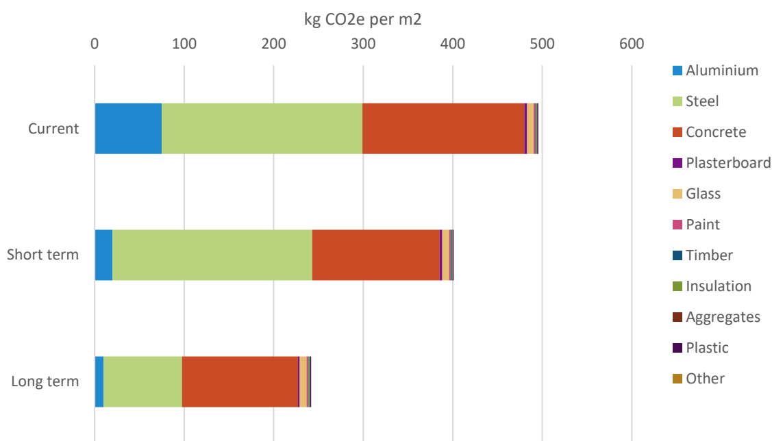
Figure 6-4: Breakdown of carbon footprint for current, short- and long-term improvements (excl. biogenic carbon) for non-residential builds
