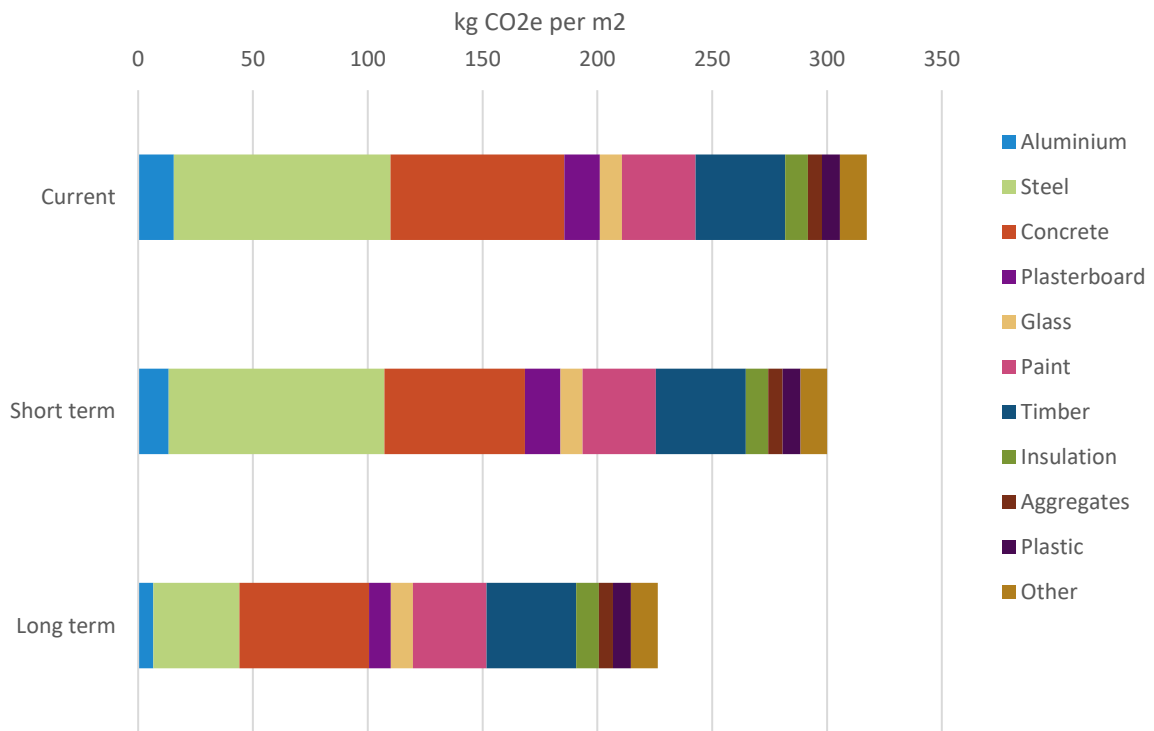
Figure 6-3: Breakdown of carbon footprint for current, short- and long-term improvements (excl. biogenic carbon) for residential builds
