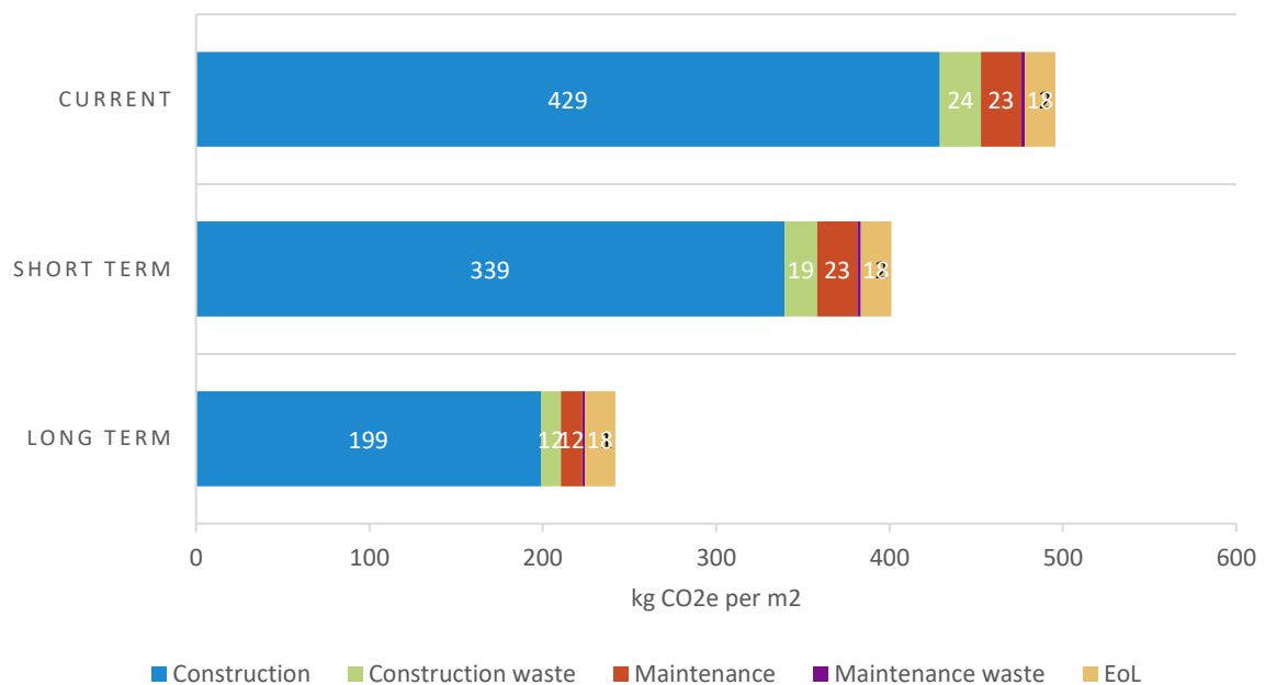
Figure 6-2: Breakdown of carbon footprint per 1 m 2 of gross floor area for non-residential builds, according to life cycle stage (excl. biogenic CO 2 )
